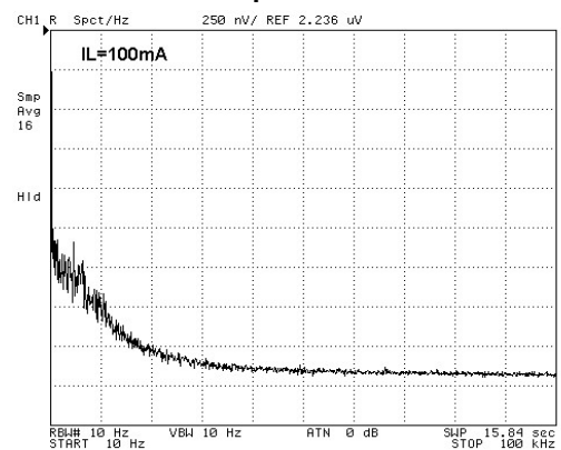
Output Noise
