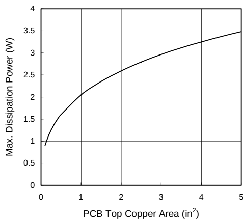
G1084T43(TO-252) Max. Power Dissipation vs. PCB Top Copper Area T_{AMB} = 25^{\circ}\text{C} ; Still Air
