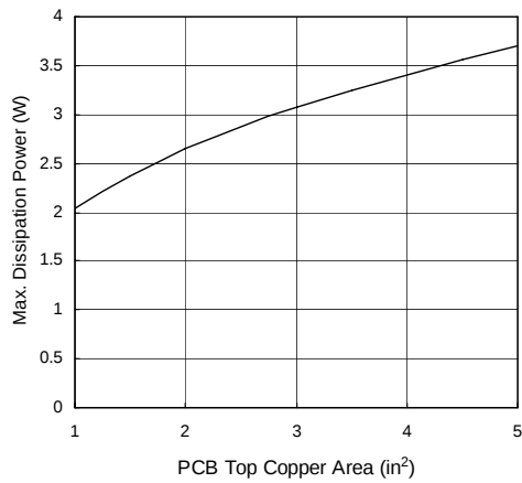
G1084T53(TO-263) Max. Power Dissipation vs. PCB Top Copper Area T_{AMB} = 25^{\circ}\text{C} ; Still Air
