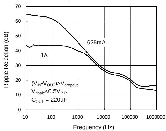
Ripple Rejection
