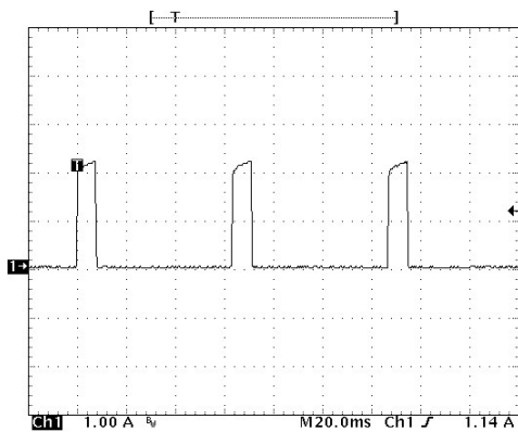
Short Circuit-Current
