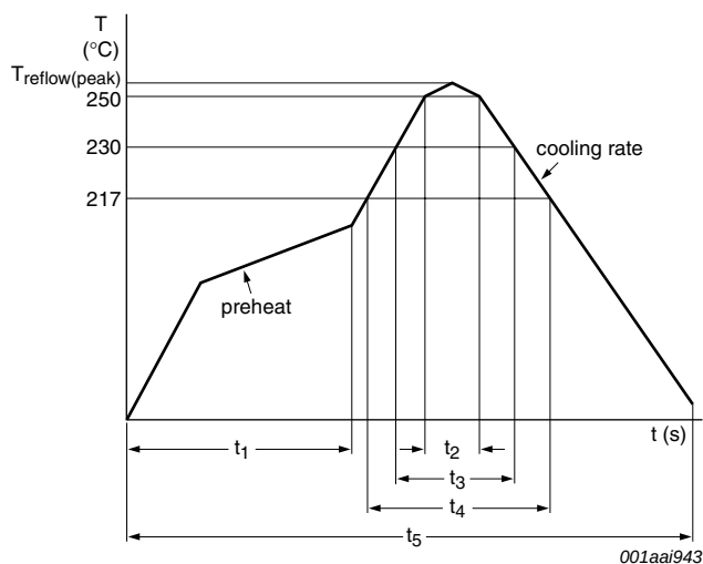
Fig 15. Pb-free solder reflow profile
