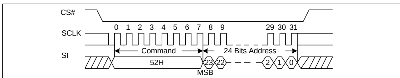
Figure 46 32KB Block Erase Sequence Diagram (ADS=0)
