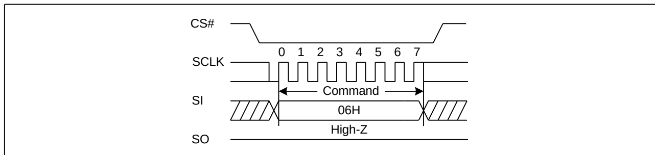
Figure 6 Write Enable Sequence Diagram
