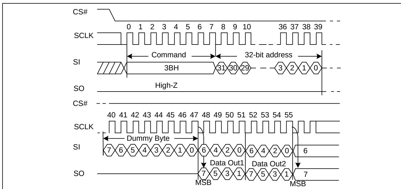
Figure 20 Dual Output Fast Read Sequence Diagram (ADS=1)
