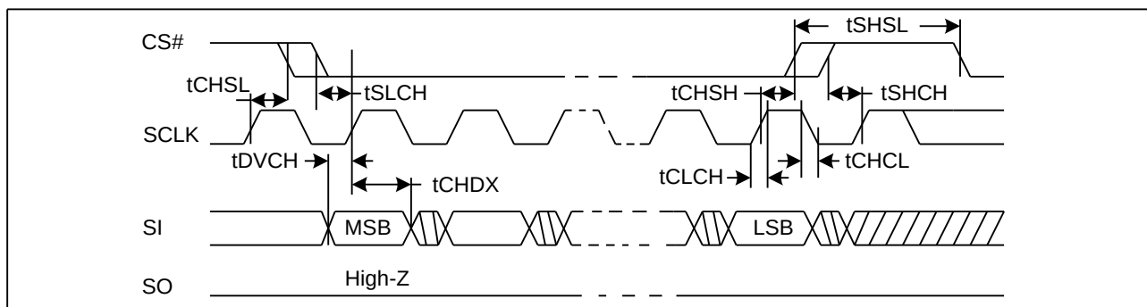
Figure 78 Serial Input Timing
