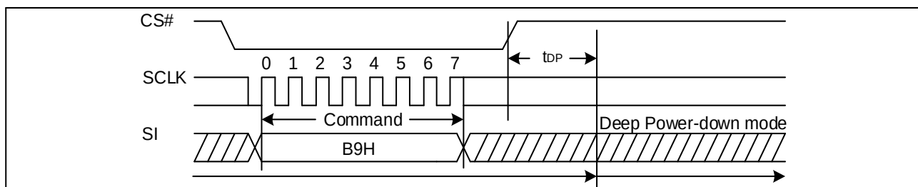
Figure 53 Deep Power-Down Sequence Diagram
