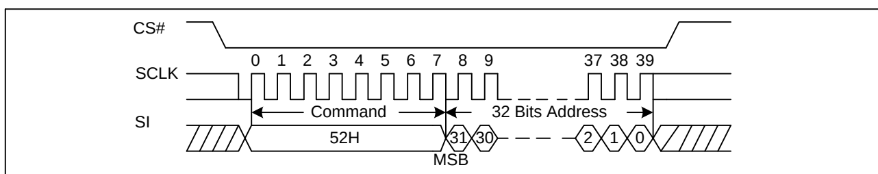
Figure 47 32KB Block Erase Sequence Diagram (ADS=1)
