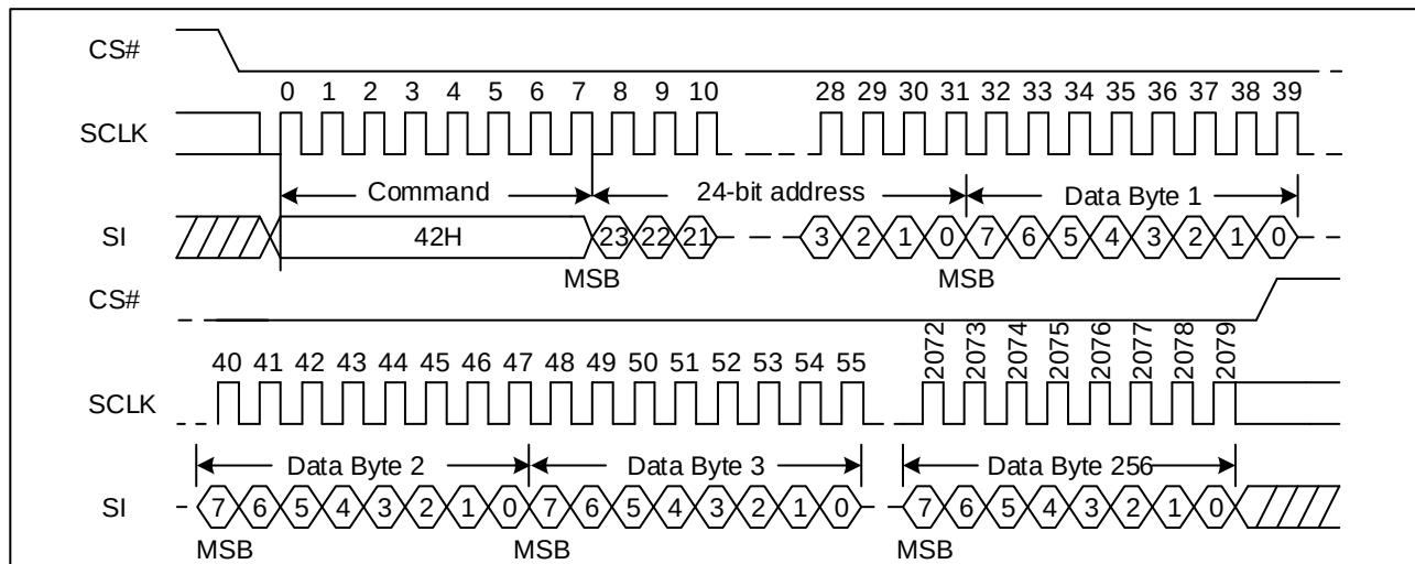
Figure 69 Program Security Registers command Sequence Diagram (ADS=0)
