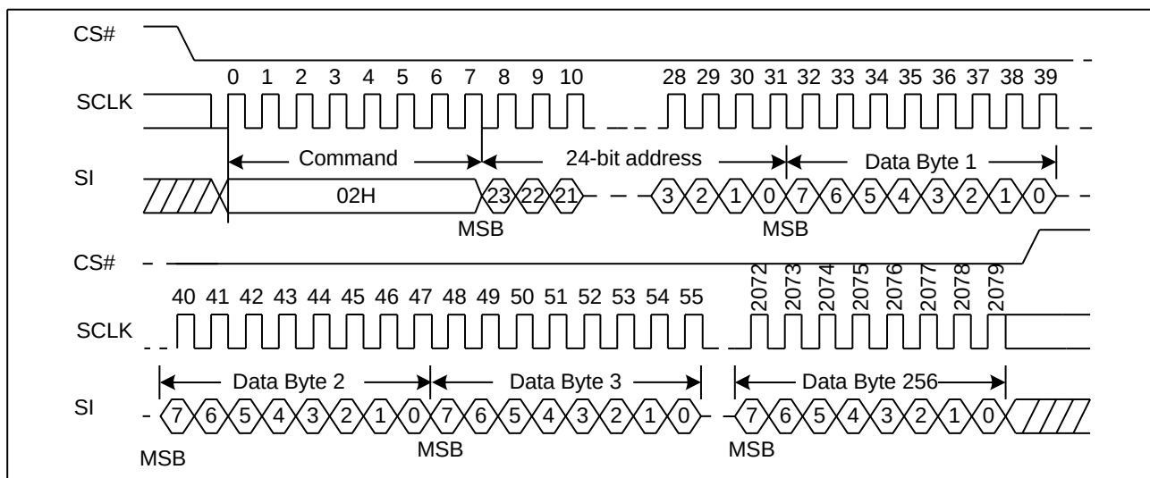
Figure 37 Page Program Sequence Diagram (ADS=0)
