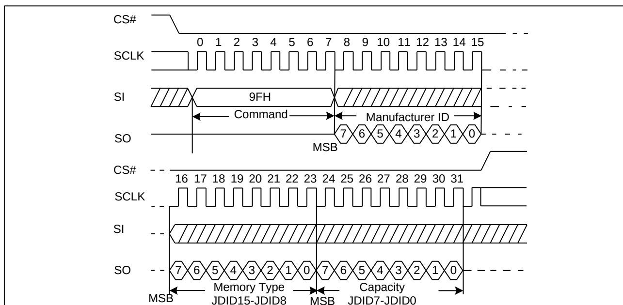
Figure 64 Read Identification ID Sequence Diagram
