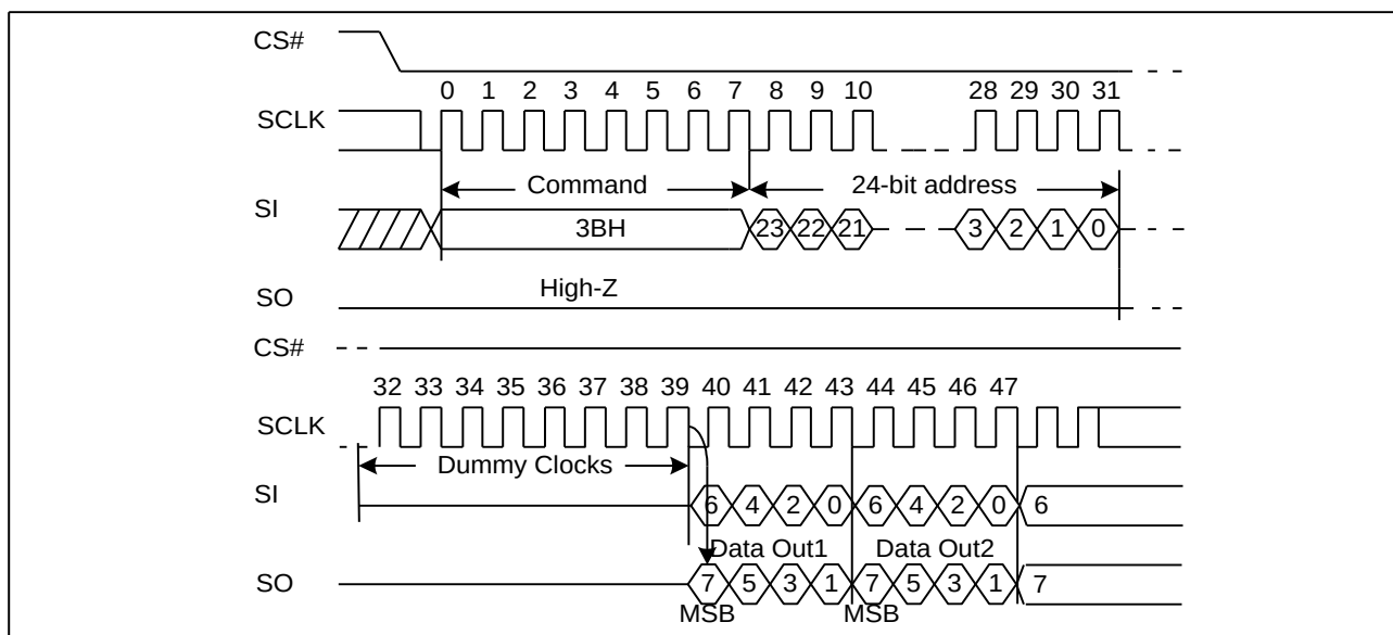
Figure 19 Dual Output Fast Read Sequence Diagram (ADS=0)
