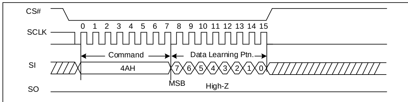
Figure 35. Write Data Learning Pattern Sequence Diagram
