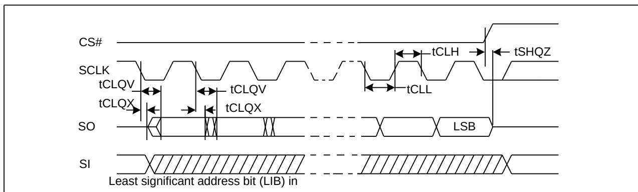
Figure 79 Output Timing
