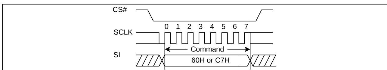
Figure 52 Chip Erase Sequence Diagram
