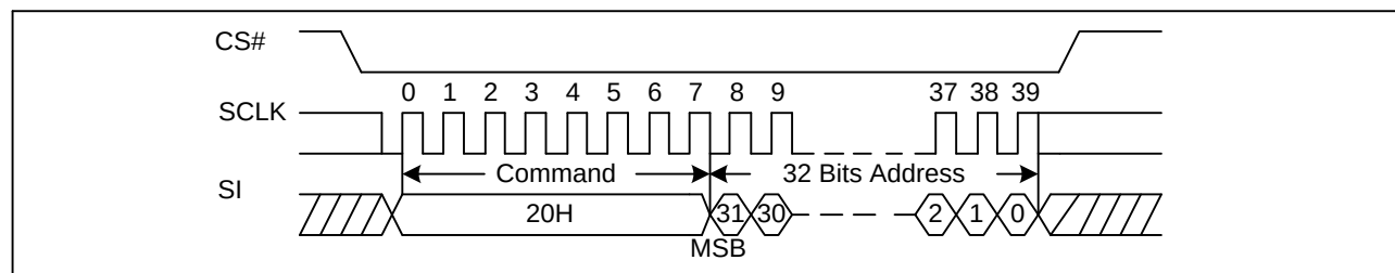
Figure 44 Sector Erase Sequence Diagram (ADS=1)
