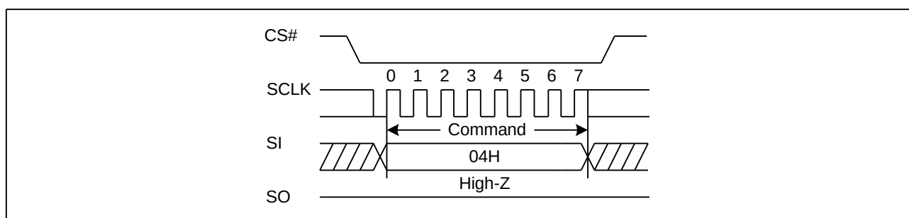
Figure 7 Write Disable Sequence Diagram
