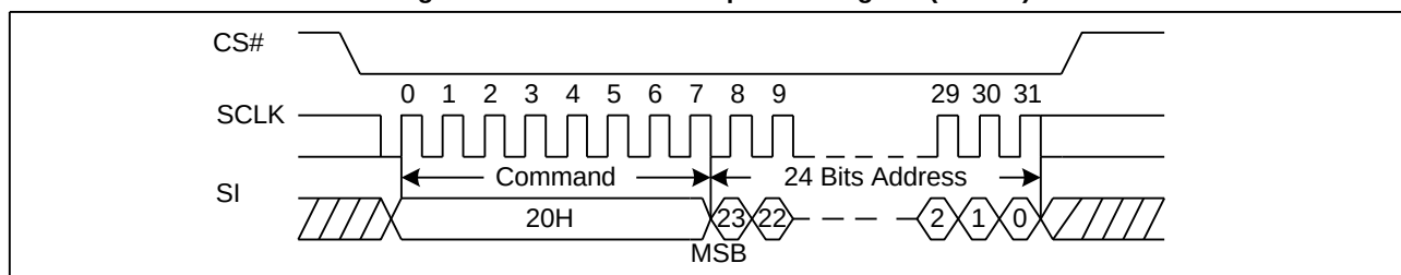
Figure 43 Sector Erase Sequence Diagram (ADS=0)
