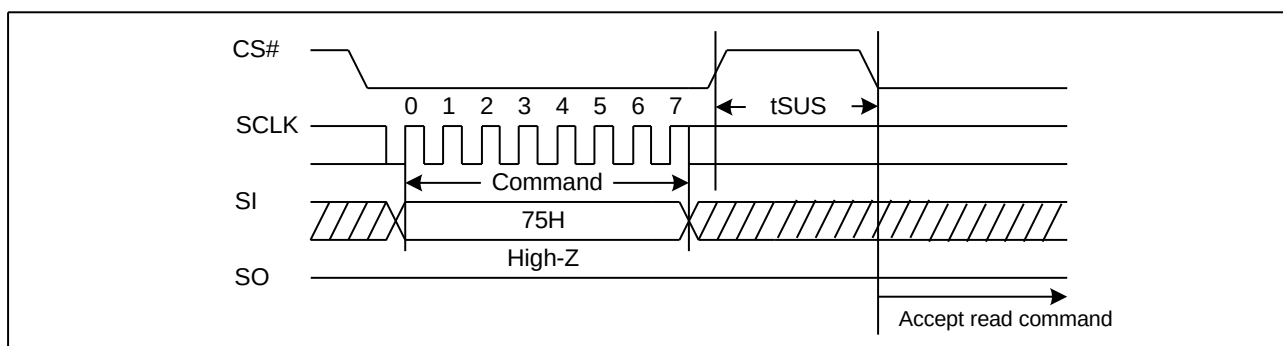
Figure 65 Program/Erase Suspend Sequence Diagram
