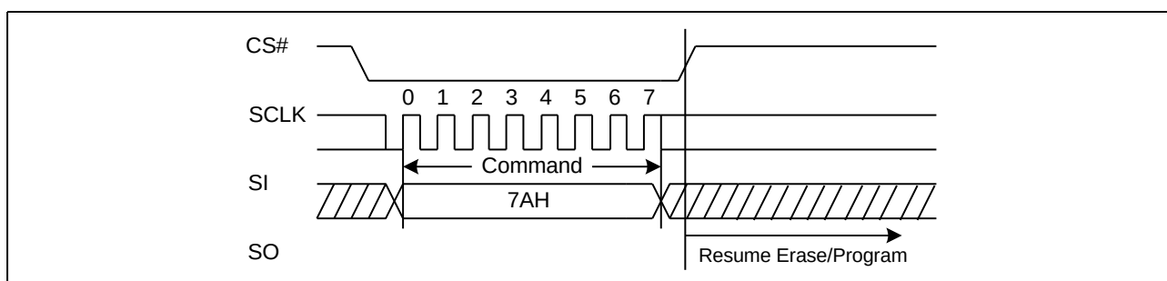
Figure 66 Program/Erase Resume Sequence Diagram
