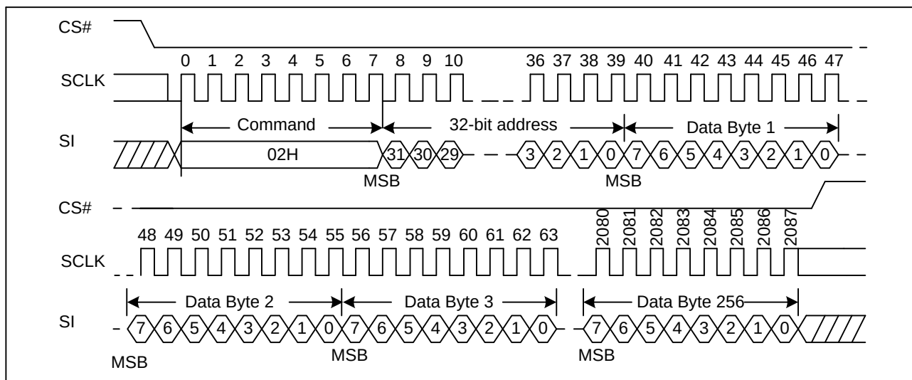
Figure 38 Page Program Sequence Diagram (ADS=1)
