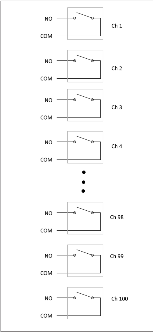
Figure 8. M9135A 20-ch, SPST, 10A, 300W
