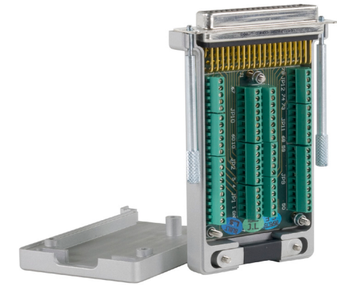
Figure 3. 78-pin Dsub connector block
