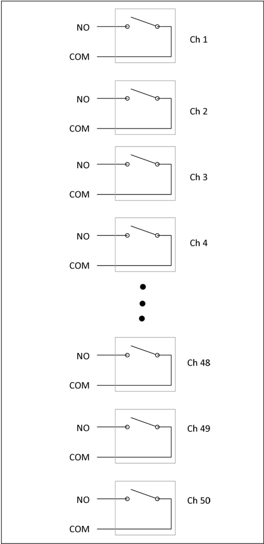
Figure 6. M9132A 50-ch, SPST, reed relays.
