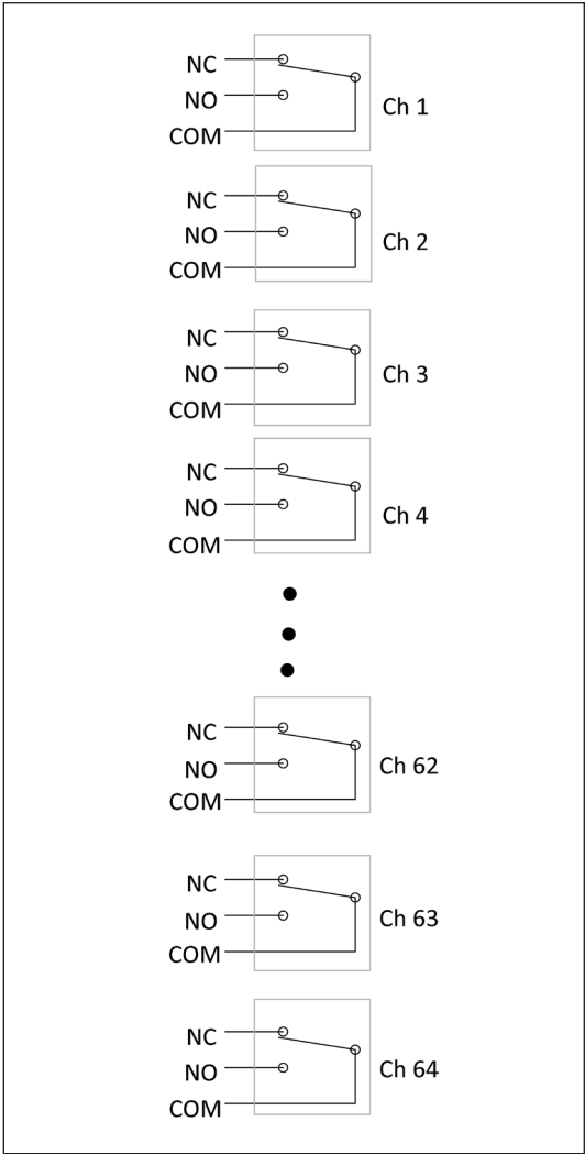
Figure 4. M9131A 64-ch, SPDT, reed relays
