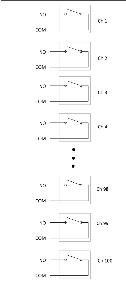
Figure 7. M9133A 100-ch, SPST, reed relays
