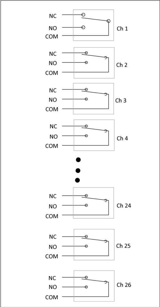
Figure 2. M9130A 26-ch, SPDT, armature relays
