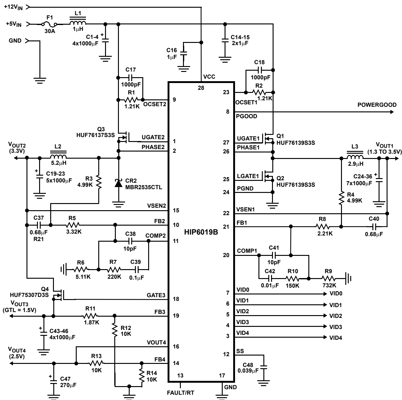
FIGURE 15. APPLICATION CIRCUIT
