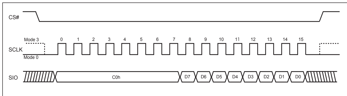
Figure 73. SPI Mode
