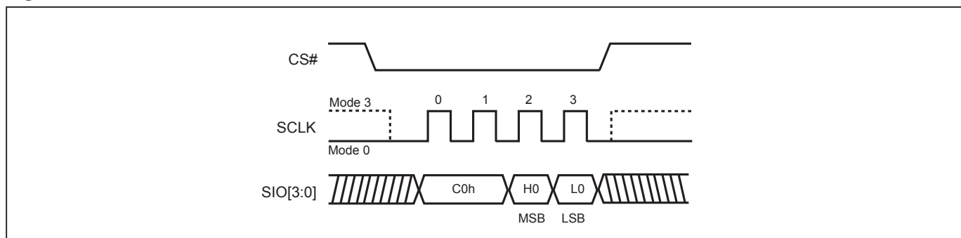
Figure 74. QPI Mode
