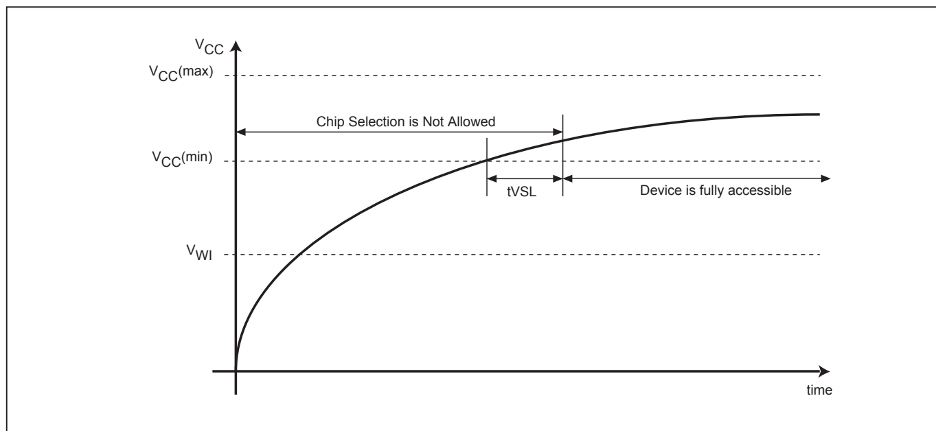
Figure 121. Power-up Timing
