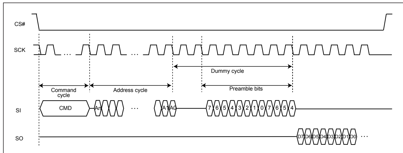
Figure 48. DTR1IO (DC=8)
