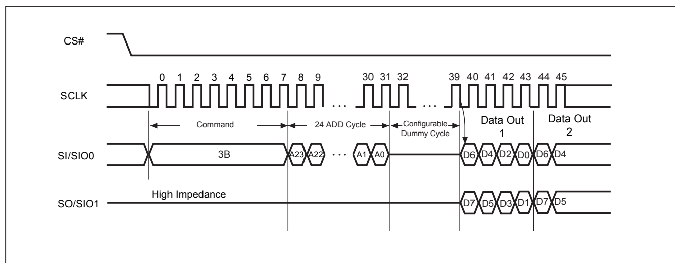
Figure 33. Dual Read Mode Sequence
