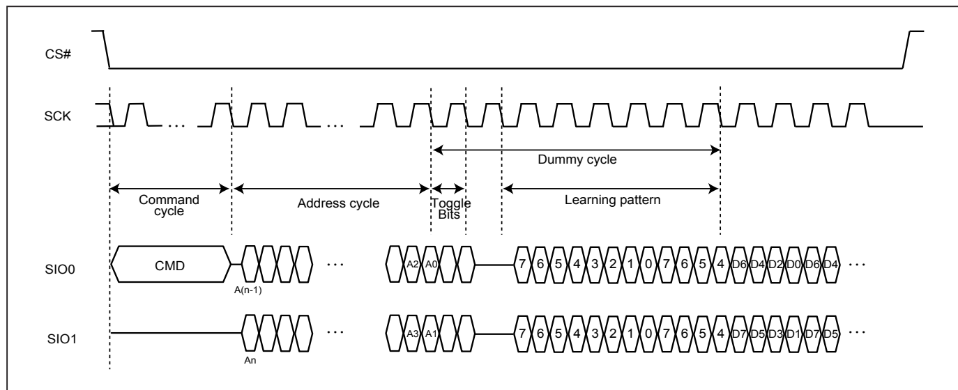
Figure 50. DTR2IO (DC=8)
