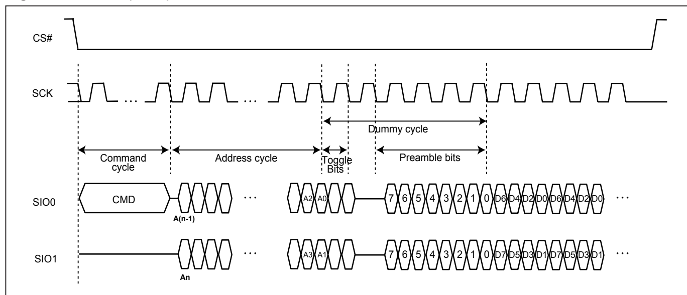
Figure 49. DTR2IO (DC=6)
