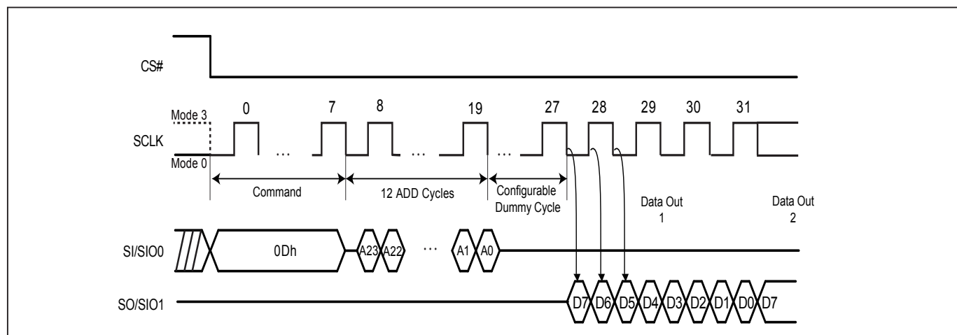
Figure 38. Fast DT Read (FASTDTRD) Sequence (SPI Only)
