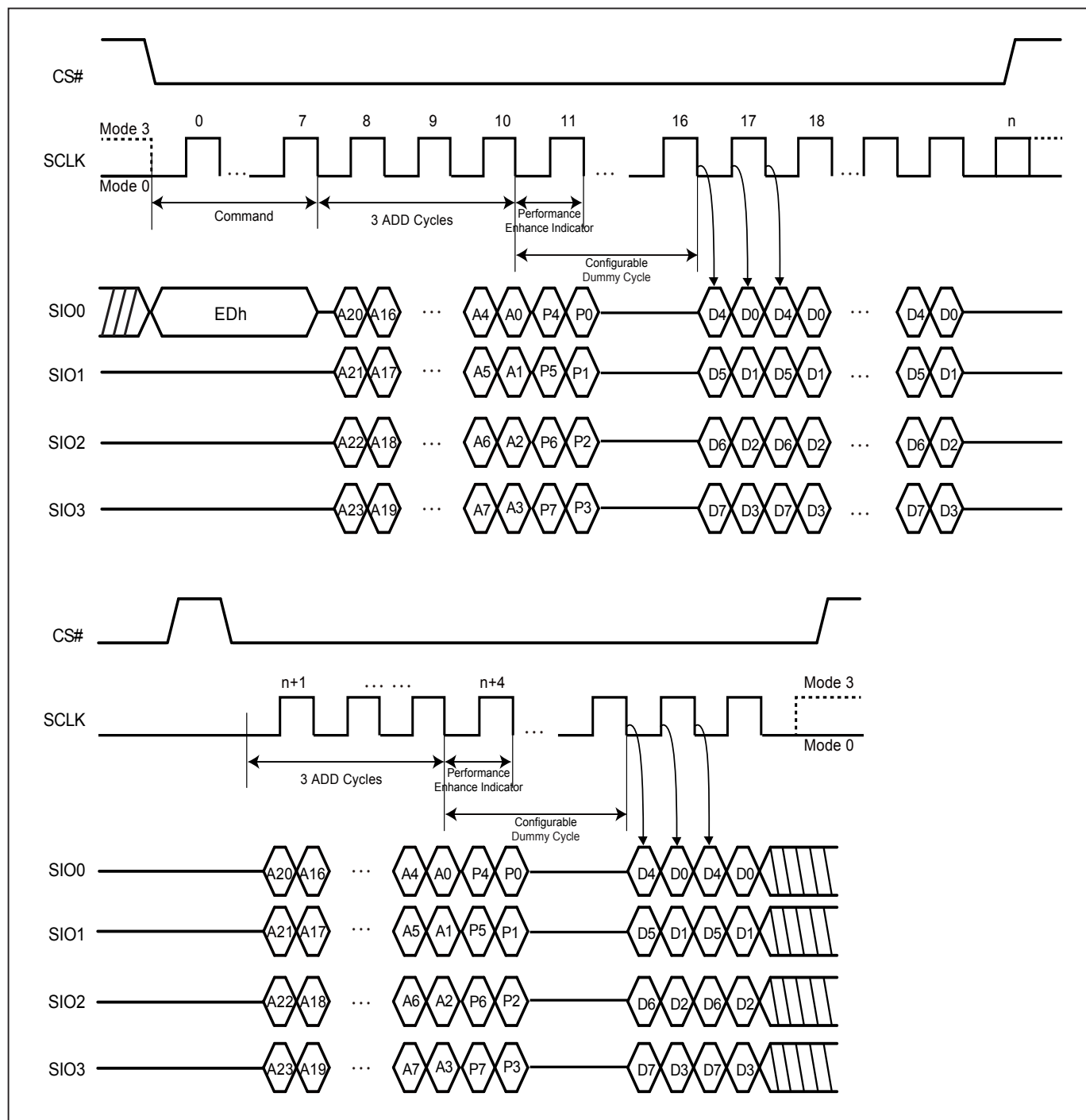
Figure 67. 4 x I/O DT Read enhance performance Mode Sequence (SPI Mode)
