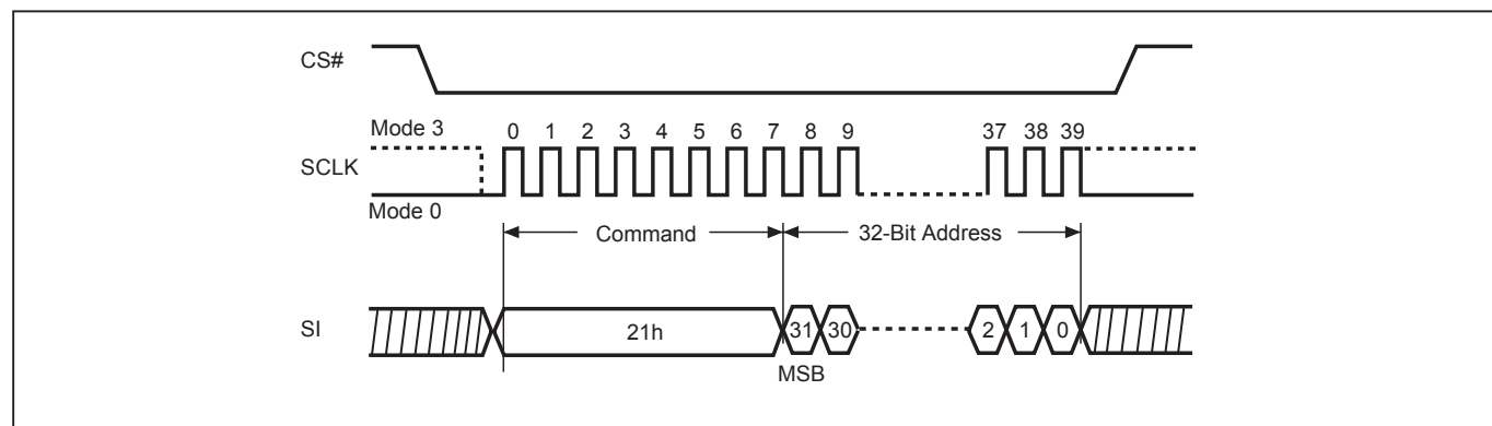
Figure 60. Sector Erase (SE4B) Sequence (SPI Mode)
