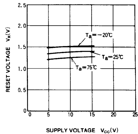
RESET VOLTAGE VS. SUPPLY VOLTAGE
