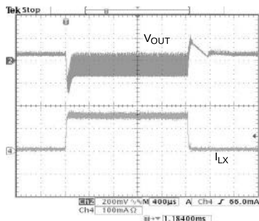
Fig. 16 Load Step Response ( V_{IN}=5V ; V_{OUT}=12V ; L1=22\mu H ; I_{OUT}=5mA to 150mA )
