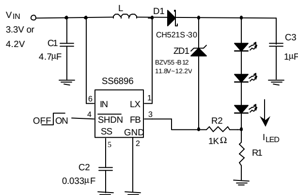
Fig. 1 Li-Ion Powered Driver for three white LEDs
