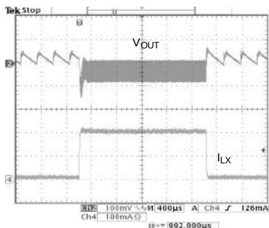
Fig. 15 Load Step Response ( V_{IN}=3.3V ; V_{OUT}=5V ; L1=10\mu H ; I_{OUT}=5mA to 200mA )
