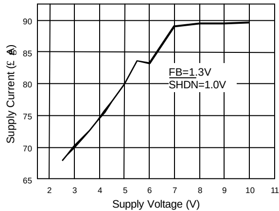
Fig. 9 Non-Switching Current
