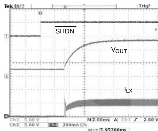
Fig. 14 Start-Up from Shutdown ( V_{IN}=3.3V ; V_{OUT}=13V ; R_{LOAD}=300\Omega )
