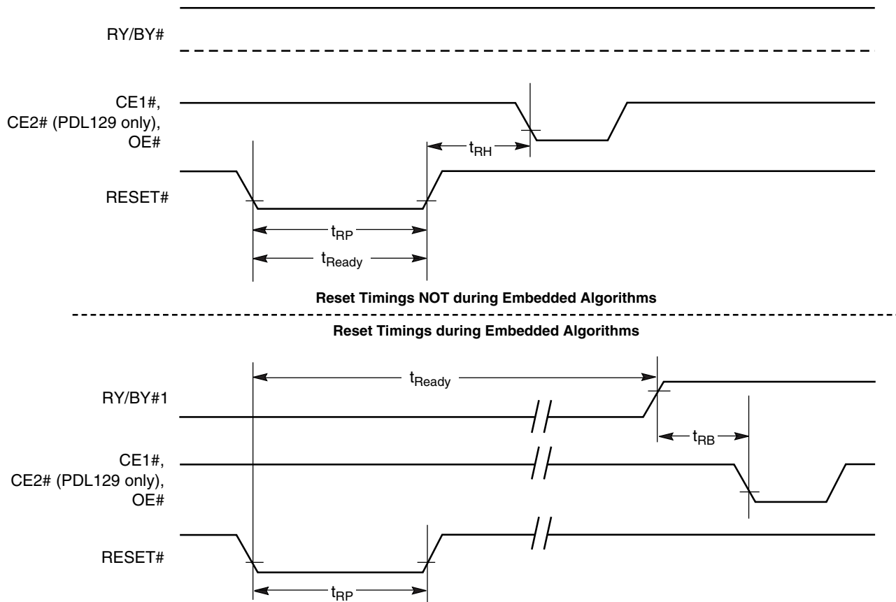
Figure 16. Reset Timings
