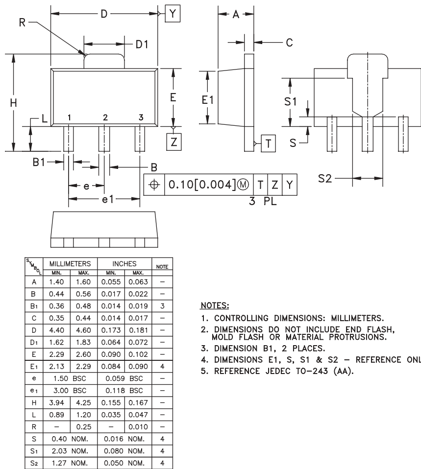
Figure 8: S24 Package Outline – SOT-89
