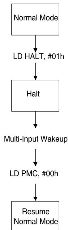
Figure 27: Recommended HALT Flow
