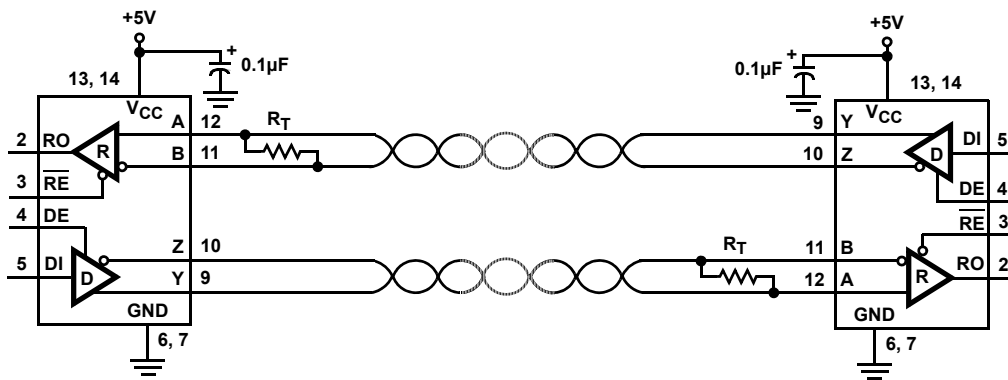
ISL32490E, ISL32493E, ISL32496E FULL DUPLEX EXAMPLE
