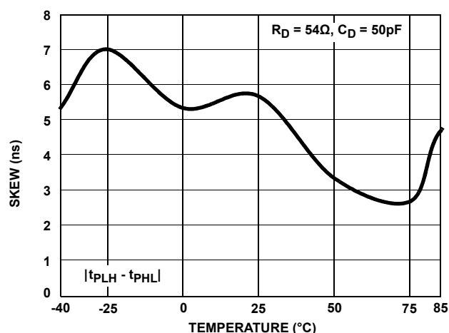
FIGURE 17. DRIVER DIFFERENTIAL SKEW vs TEMPERATURE (ISL32490E, ISL32492E)
