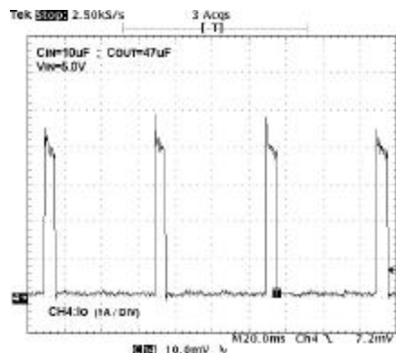
Short Circuit-Current
