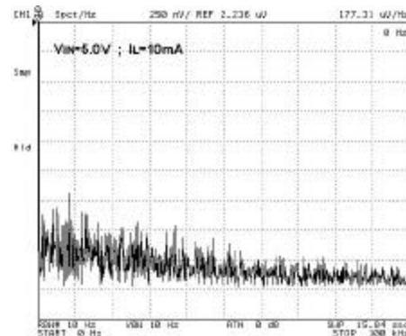
Output Noise
