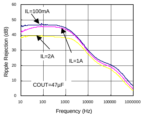
Ripple Rejection
