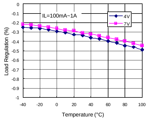
Load Regulation
