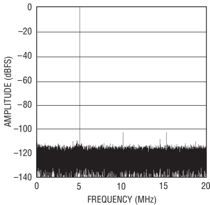
LTC2204: 64K Point FFT, 40Msps, f_{IN} = 5.1\text{MHz} , -1dBFS, PGA = 1, DITH = 0
