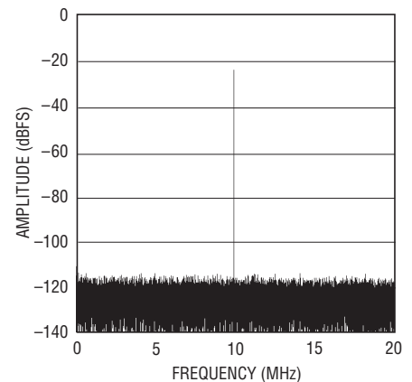
LTC2204: 64K Point FFT, 40Msps, f_{IN} = 70.1\text{MHz} , -25\text{dBFS} , PGA = 0, DITH = 1
