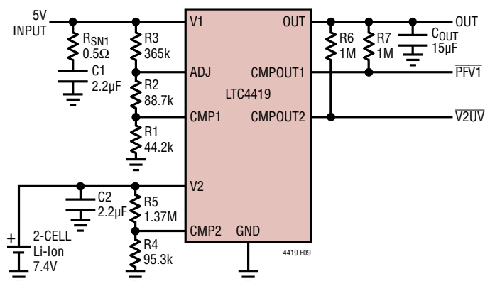
Figure 9. Design Example
