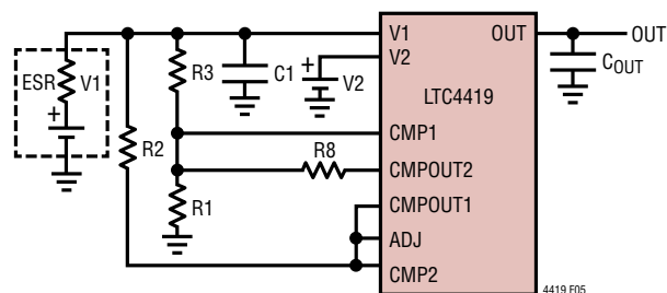
Figure 5. Increasing Supply Hysteresis in High ESR Applications
