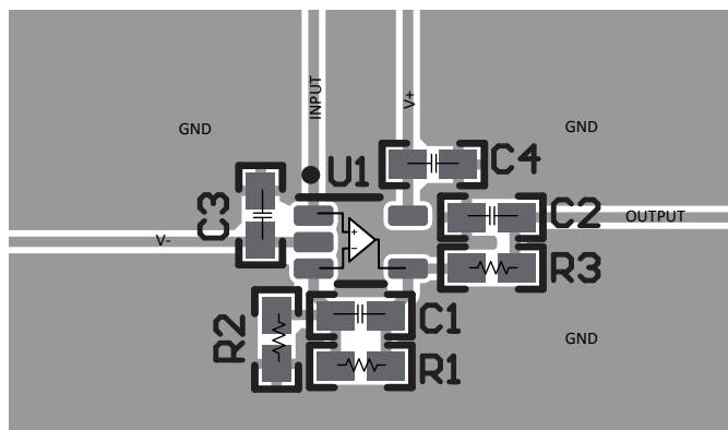
Figure 5. Operational Amplifier Board Layout for Noninverting Configuration
