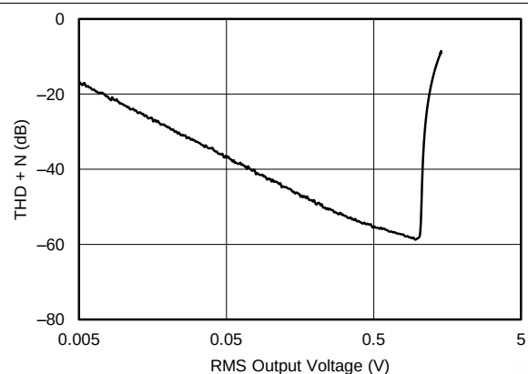
Figure 4. THD + N vs RMS Output Voltage
