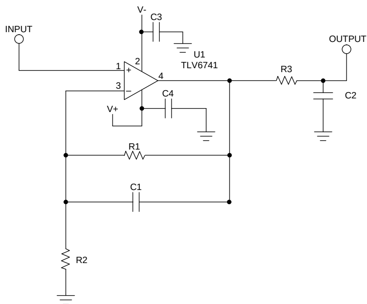
Figure 6. Schematic Used for Layout Example
