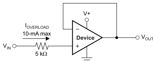
Figure 1. Input Current Protection
