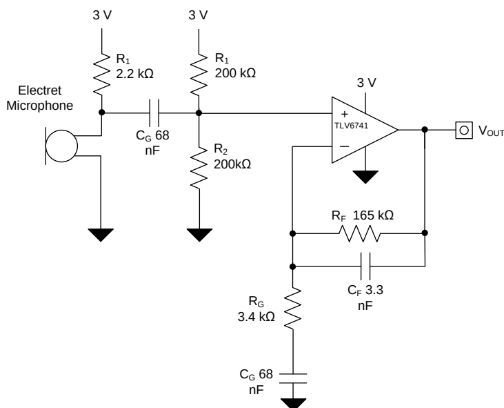
Figure 2. Microphone pre-amplifier
