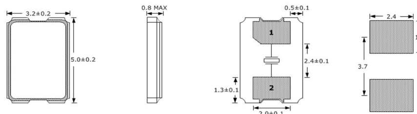
ELECTRODE ARRANGEMENT (BOTTOM VIEW)
