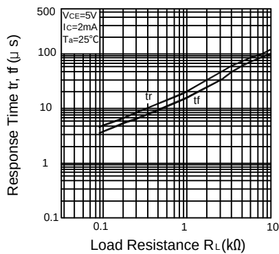
Response Time vs. Load Resistance
