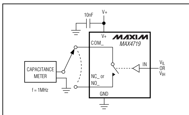
Figure 5. Channel Off/On-Capacitance
