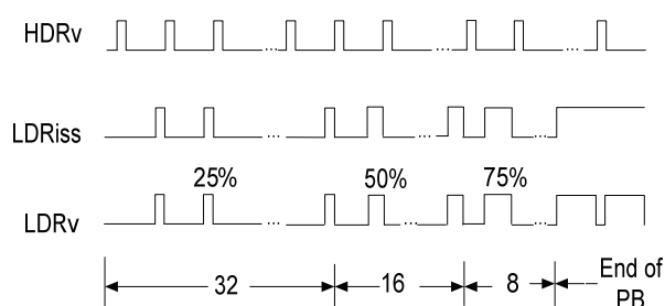
Fig. 5b. Pre-Bias startup pulses
