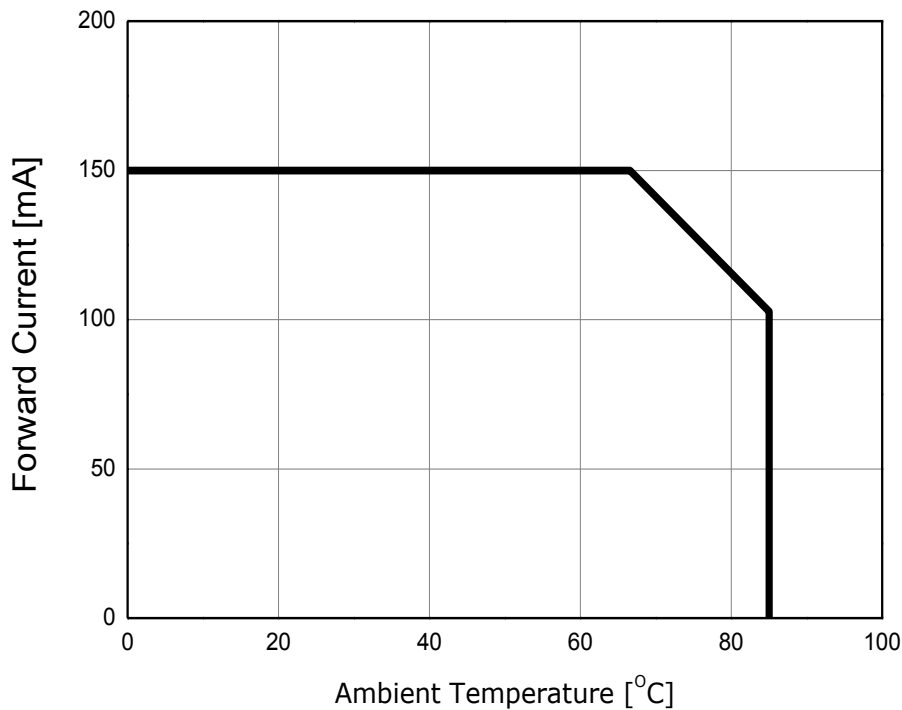
Fig 4. Ambient Temperature vs. Maximum Forward Current, T j,max = 125°C
