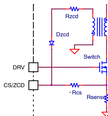
Figure 8. ZCD Winding Implementation
