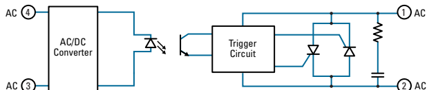
Diagram: A48xxT
