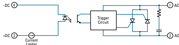
Diagram: D48xxT
