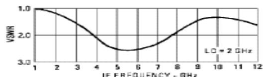
I-Port VSWR vs. Frequency, LO @ +10 dBm
