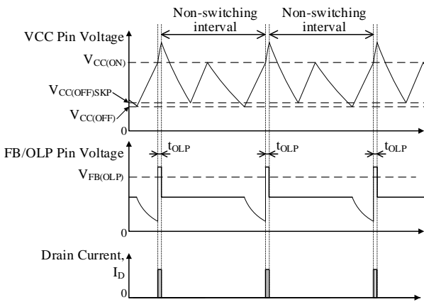
Figure 9-16. OLP Operational Waveforms
