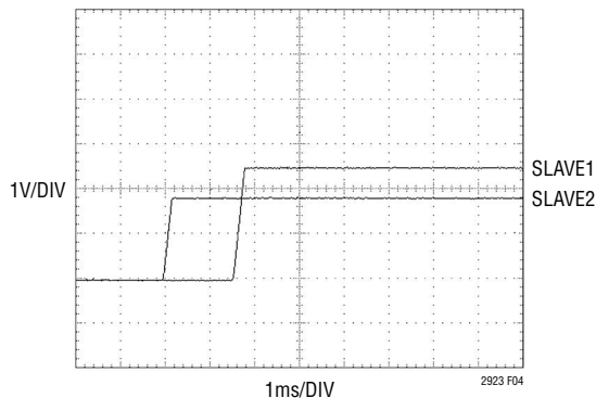
Figure 4. Supply Sequencing
