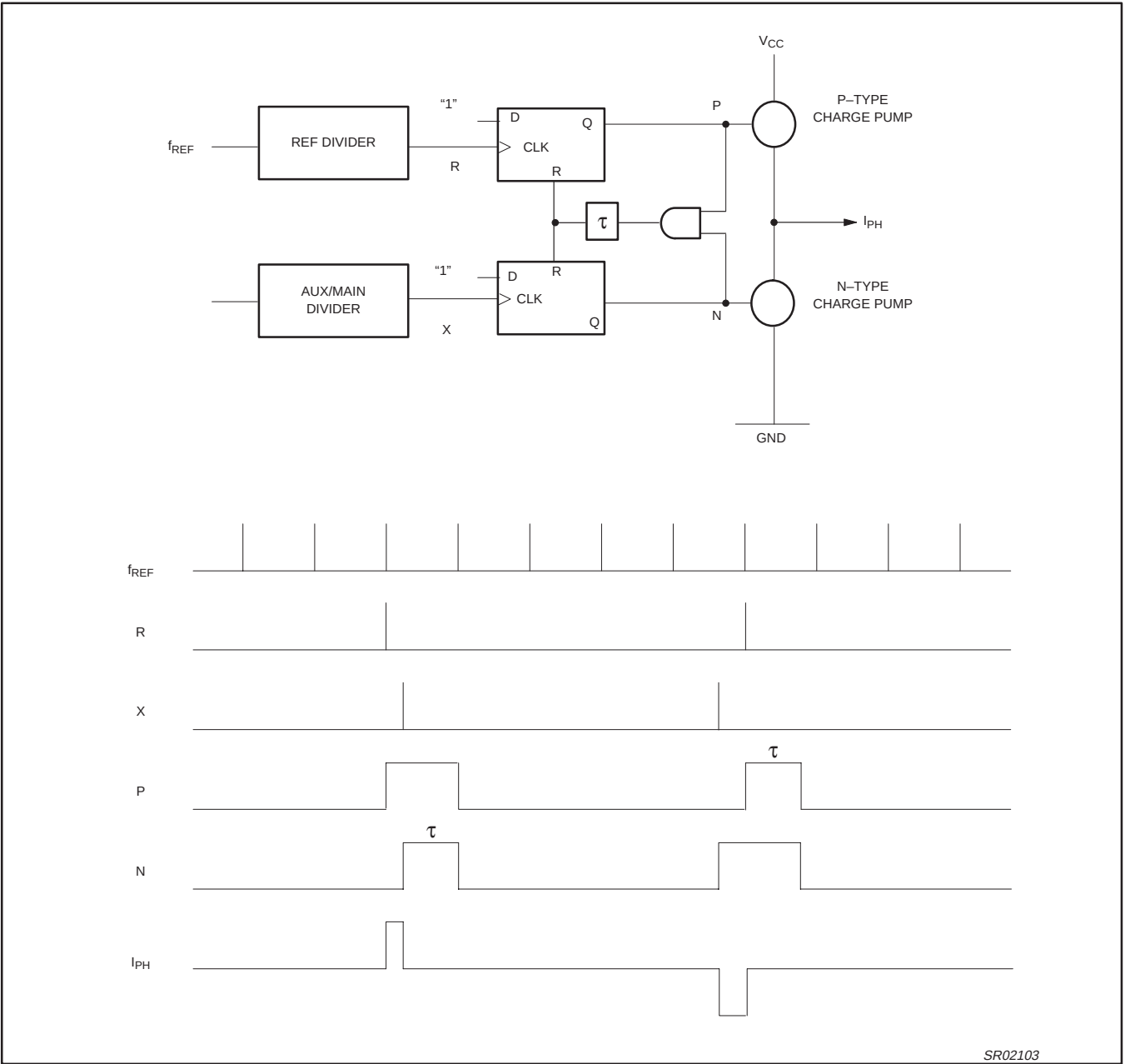
Figure 5. Phase Detector Structure with Timing
