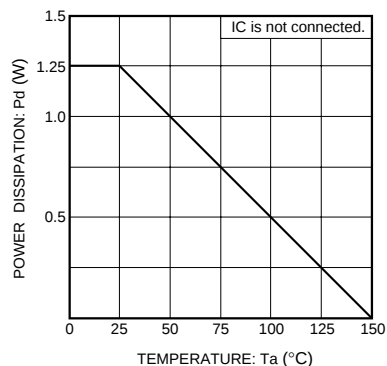
Fig. 3 Power dissipation
