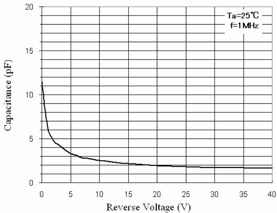
Total Capacitance
