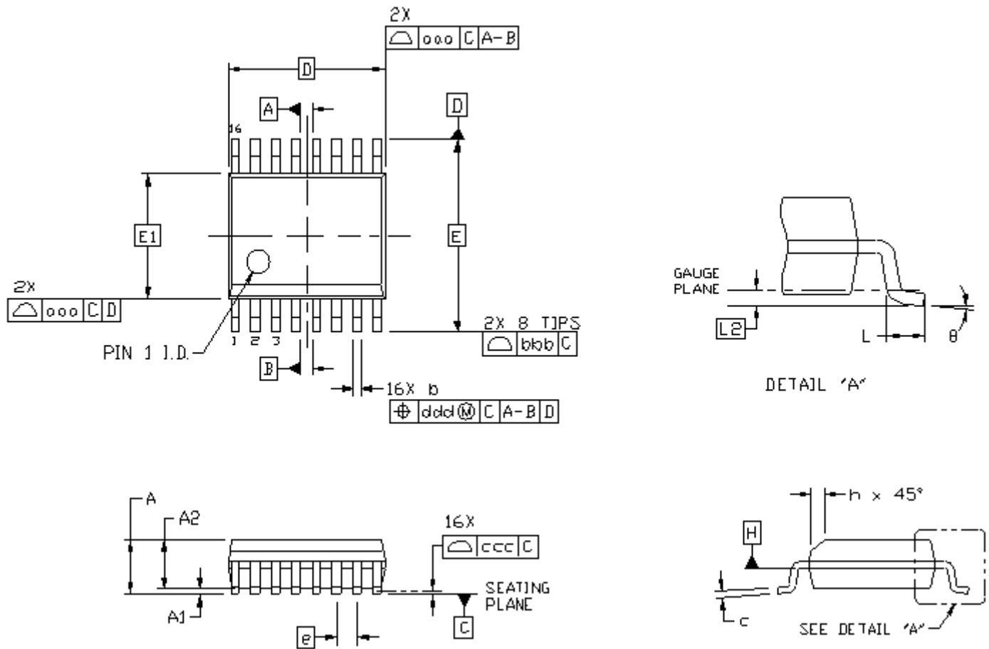
Figure 10.1. 16-Pin QSOP
