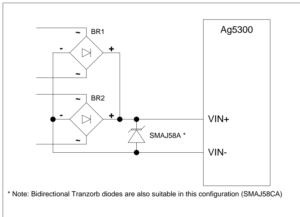
Figure 13: Input Protection
