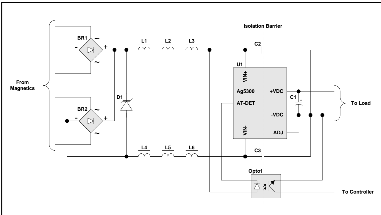
Figure 14:EMC Filtering
