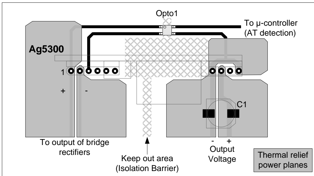
Figure 12: Thermal Relief Power Planes
