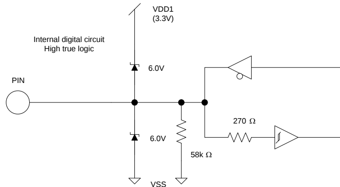
Figure 13 PWMUL/PWMUH/PWMVL/PWMVH/PWMWL/PWMWH output
