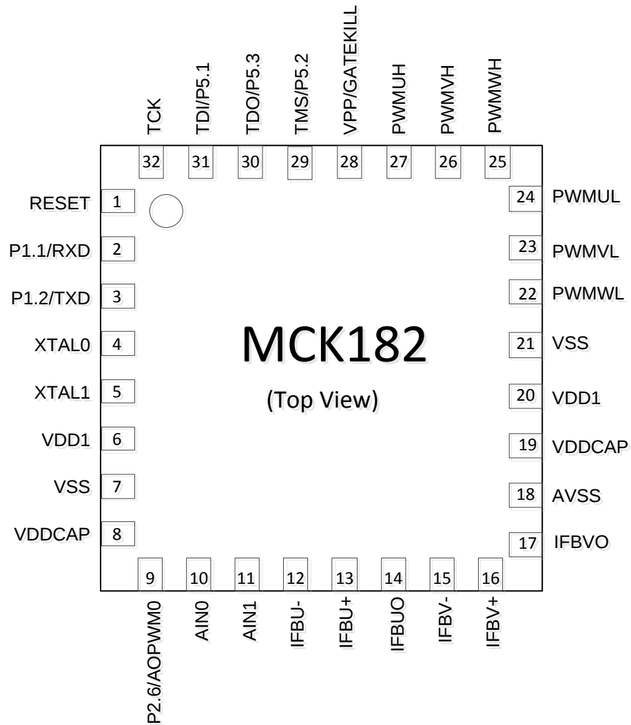
Figure 2 Pinout of IRMCK182M
