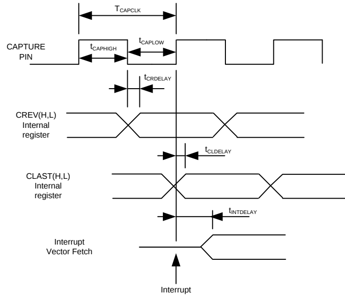
Figure 10 CAPTURE timing
