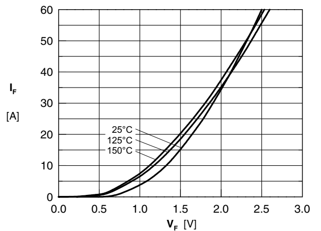
Fig. 18 Forward characteristics boost diode
