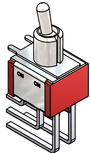
ISOMETRIC
