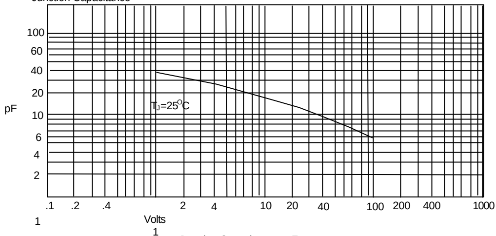
Figure 3 Junction Capacitance
