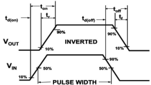
Figure 2: Switching Waveforms
