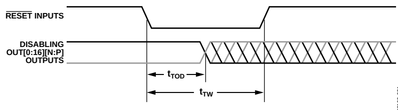
Figure 31. Asynchronous Reset
