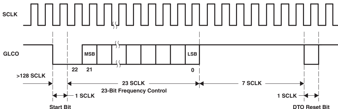
Figure 3-9. GLCO Timing
