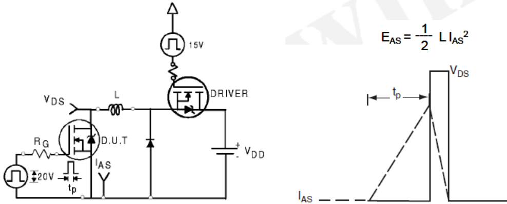
Fig. 16. Unclamped Inductive switching test circuit & waveform
