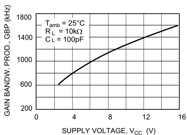
Figure 9. Gain bandwidth product vs. supply voltage
