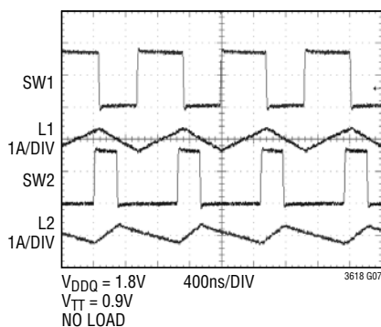
Forced Continuous Mode Operation (FCM)
