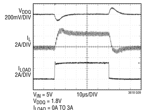
Load Step Transient with FCM Internal Compensation
