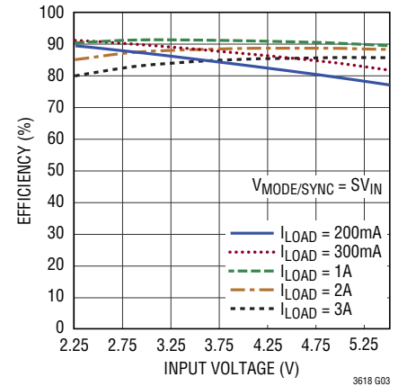
Efficiency vs Input Voltage V_{DDQ} = 1.8\text{V}
