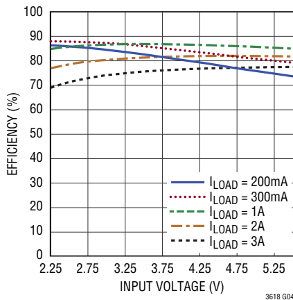
Efficiency vs Input Voltage V_{TT} = 0.9\text{V}
