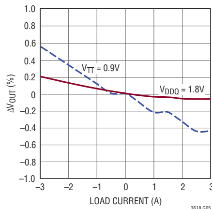
VOUT Load Regulation
