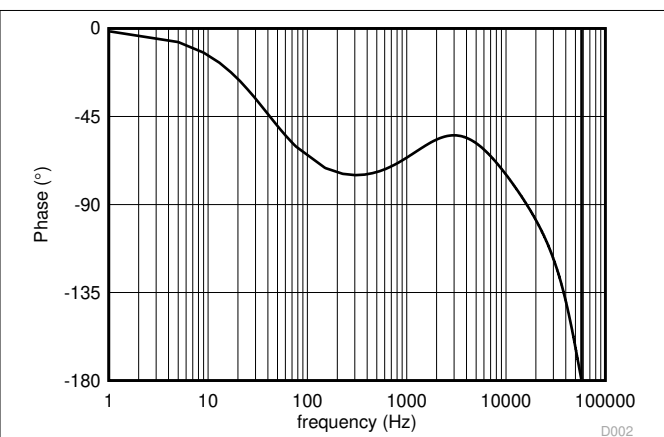
Figure 9-5. Converter Open-Loop Bode Plot - Phase
