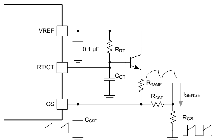
Figure 8-5. Oscillator Synchronization Circuit
