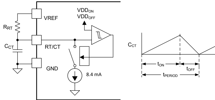
Figure 8-4. Oscillator Circuit
