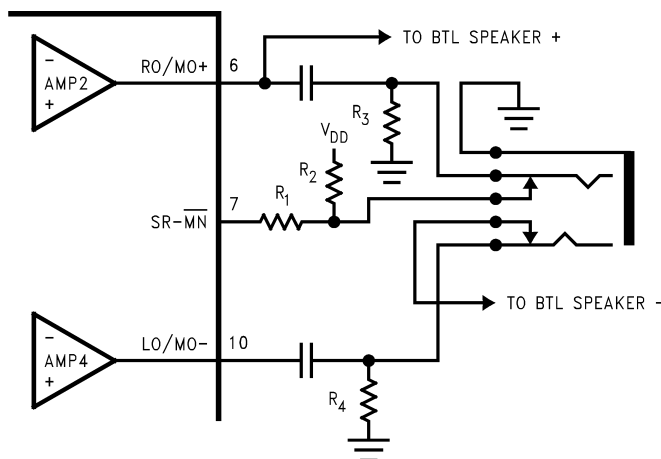
FIGURE 4. Headphone Circuit
