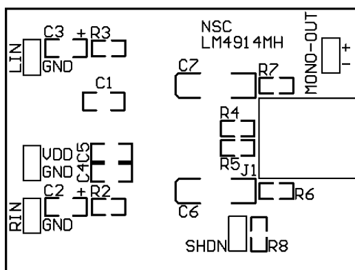
FIGURE 5. Top Overlay
