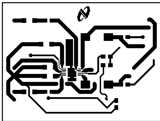
FIGURE 6. Top Layer
