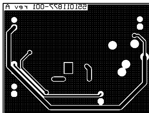
FIGURE 7. Bottom Layer
