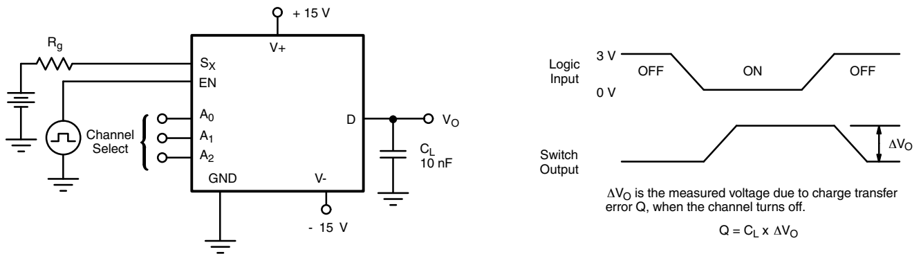
Fig. 5 - Charge Injection
