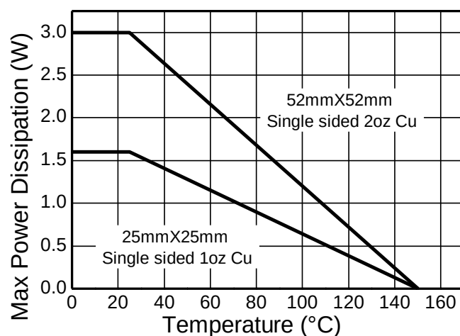
Derating Curve
