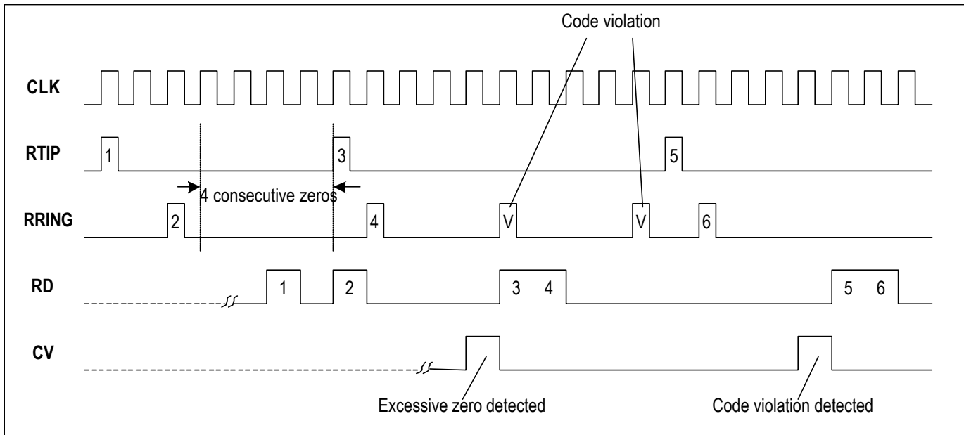
Figure - 8. HDB3 Code Violation &amp; Excessive Zero
