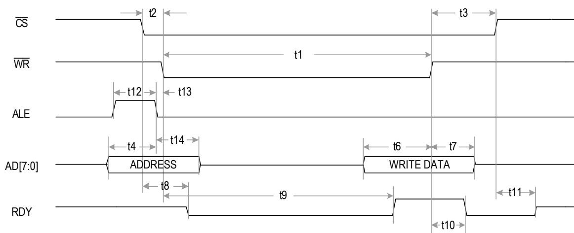
Figure - 30. Multiplexed Intel Mode Write Timing
