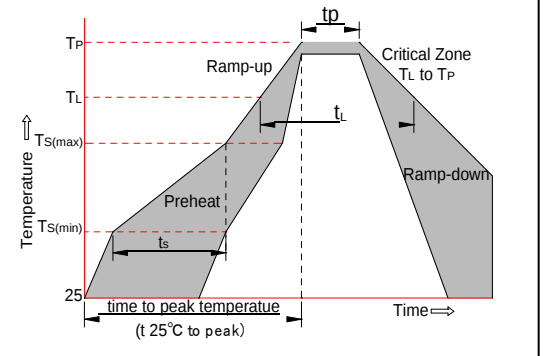
FIG.5: Reflow condition
