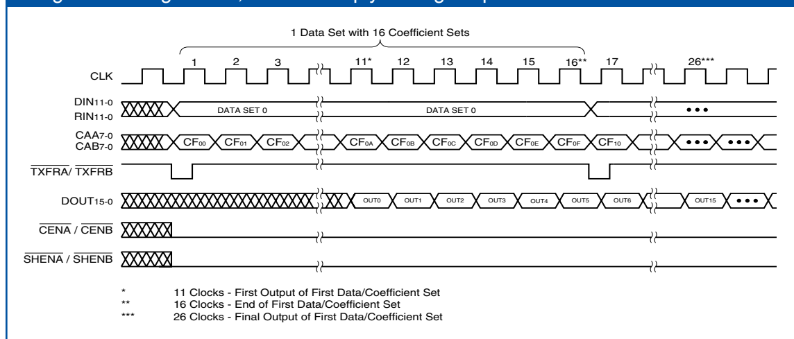
Figure 20. Single Filter, Matrix Multiply Timing Sequence
