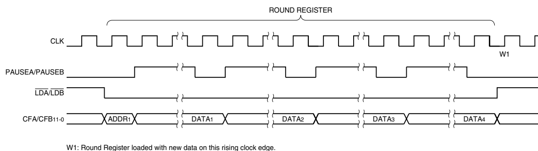
Figure 13. Round Register Loading Sequence with PAUSE Implementation
