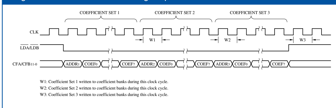
Figure 9. Coefficient Bank Loading Sequence
