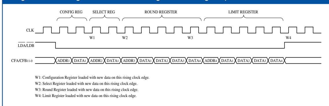
Figure 10. Configurational/Control Register Loading Sequence
