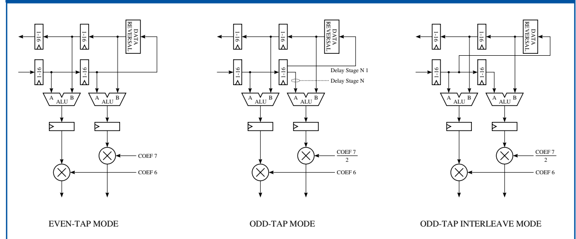
Figure 5. I/D Register Data Paths
