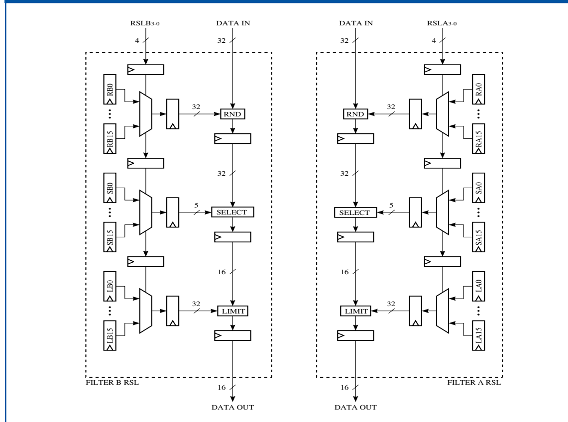
Figure 7 .Filter A and Filter B Round/Limit/Select Circuitry
