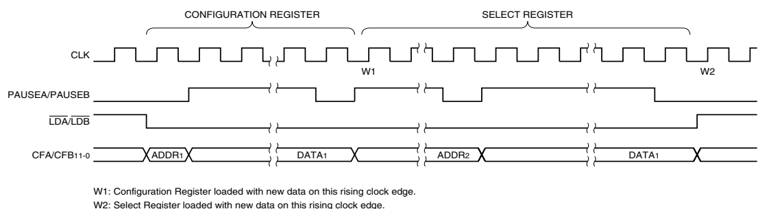
Figure 12. Config and Select Register Loading Sequence w/ PAUSE Implementation
