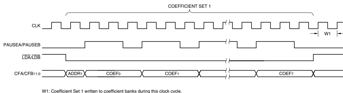
Figure 11. Coefficient Bank Loading Sequence with PAUSE Implementation
