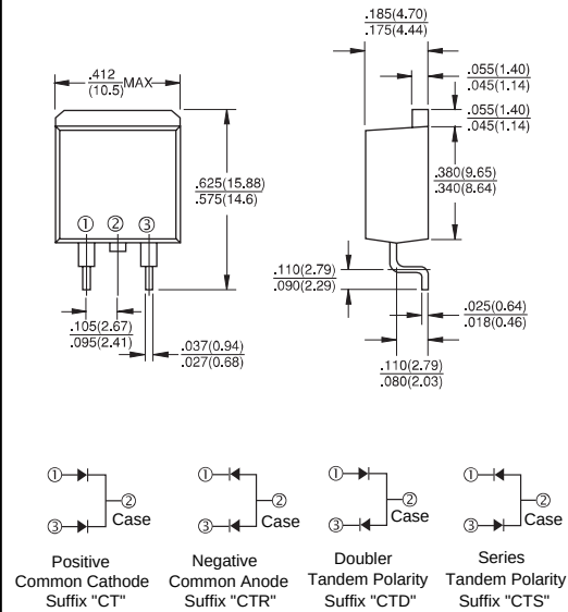
D2PAK/TO-263
