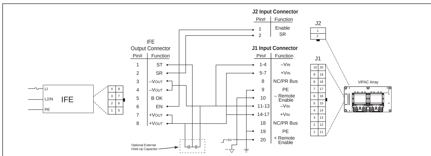
Figure 4 —Connection diagram using IFE with ViPAC Array
